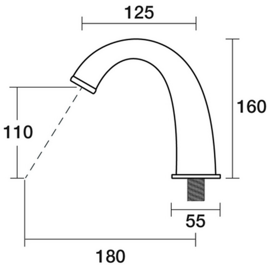
Tudor Basin Deluxe Outlet D31.014.1.23 - Gunmetal
