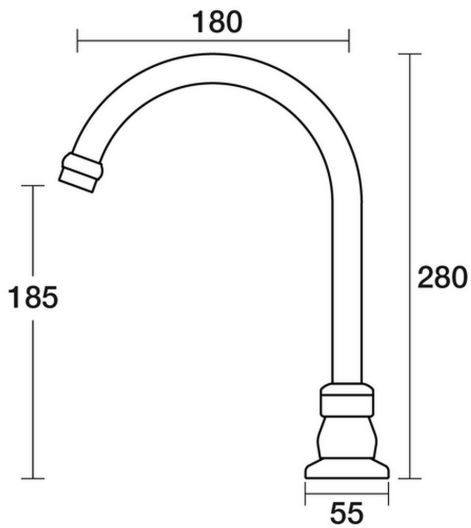
Tudor Sink Hob Swivel Outlet D31.032.1.57 - Matt Nickel
