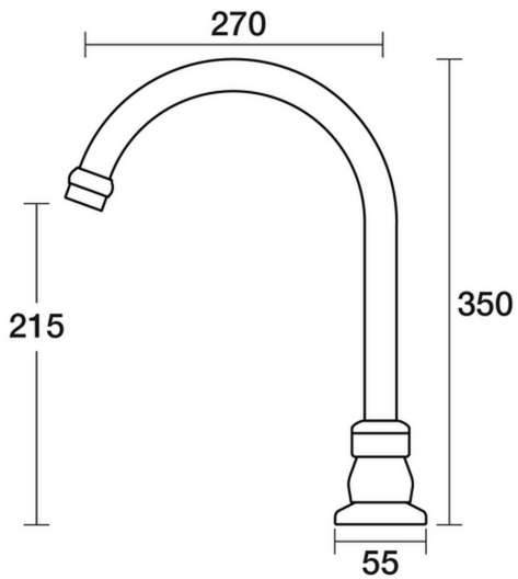
Tudor Sink Hob Swivel Outlet X/Large D31.032.2.07 - Chrome / Victorian Green
