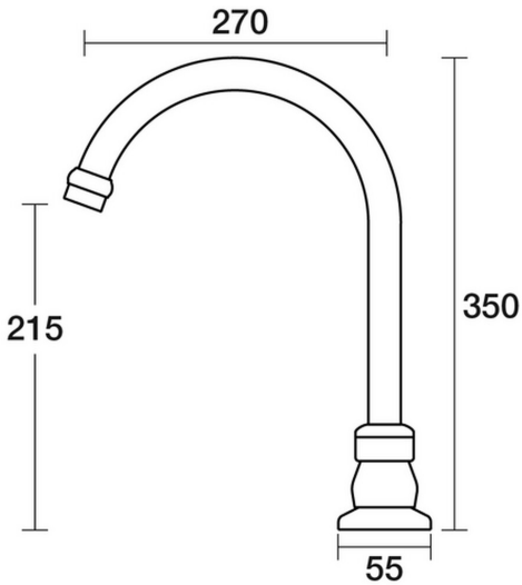
Tudor Sink Hob Swivel Outlet X/Large D31.032.2.23 - Gunmetal
