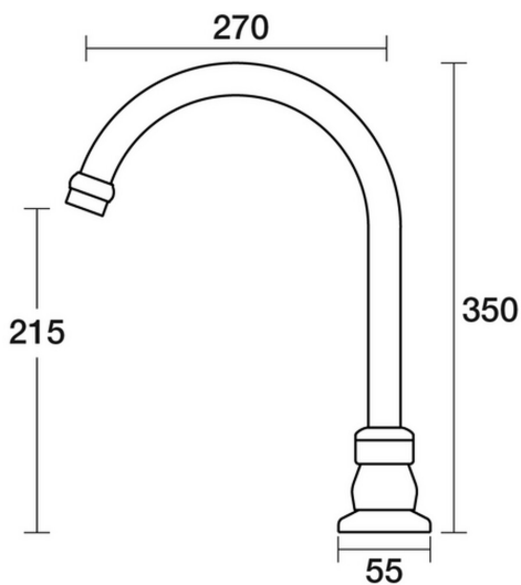
Tudor Sink Hob Swivel Outlet X/Large D31.032.2.26 - Black Sapphire
