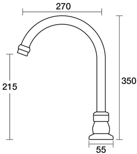
Tudor Sink Hob Swivel Outlet X/Large D31.032.2.45 - Native Brass
