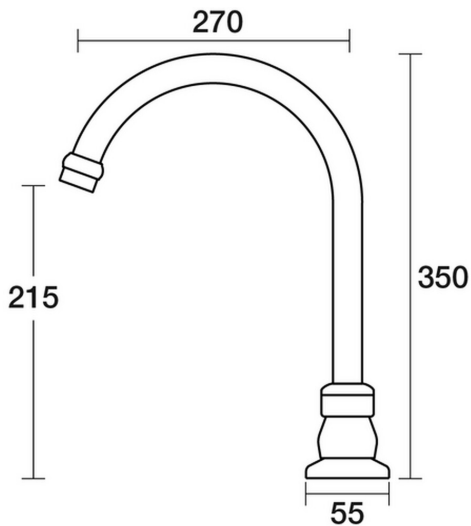
Tudor Sink Hob Swivel Outlet X/Large D31.032.2.57 - Matt Nickel
