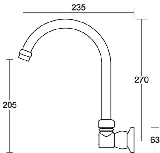
Tudor Sink Wall Swivel Outlet D31.034.1.02 - Brushed Chrome
