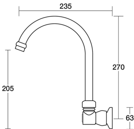
Tudor Sink Wall Swivel Outlet D31.034.1.57 - Matt Nickel
