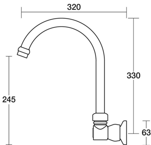
Tudor Sink Wall Swivel Outlet X/Large D31.034.2.06 - Chrome / Sienna Red
