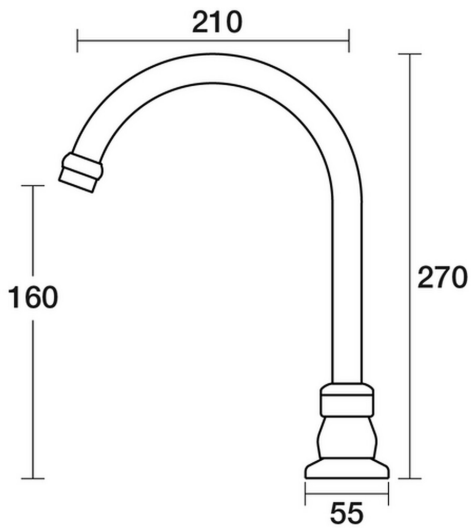
Tudor Spa Hob Swivel Outlet D31.042.1.45 - Native Brass
