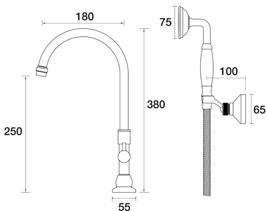
Tudor Spa Hob Swivel Outlet Divertor Outlet with Handshower & Bracket D31.042.2.15 - Gold / Apricot
