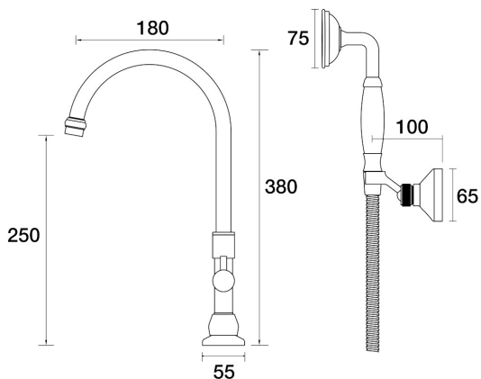
Tudor Spa Hob Swivel Outlet Divertor Outlet with Handshower & Bracket D31.042.2.26 - Black Sapphire
