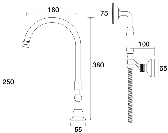
Tudor Spa Hob Swivel Outlet Divertor Outlet with Handshower & Bracket D31.042.2.57 - Matt Nickel
