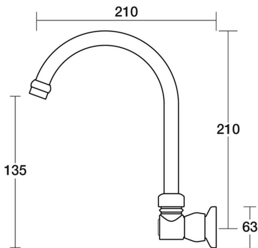
Tudor Spa Wall Swivel Outlet D31.044.1.02 - Brushed Chrome
