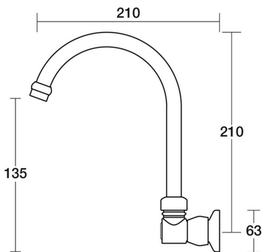
Tudor Spa Wall Swivel Outlet D31.044.1.12 - 23k Brushed Gold
