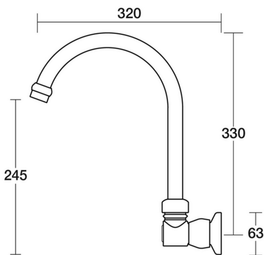
Tudor Spa Wall Swivel Outlet X/Large D31.044.2.43 - Brass
