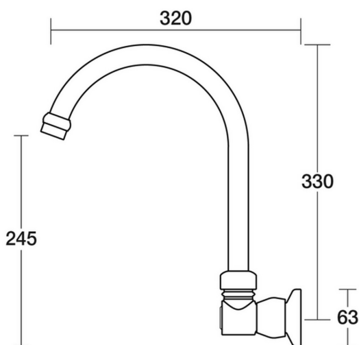
Tudor Spa Wall Swivel Outlet X/Large D31.044.2.47 - Luminick
