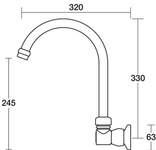
Tudor Spa Wall Swivel Outlet X/Large D31.044.2.67 - Vintage Brass
