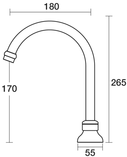
Bell Sink Hob Swivel Outlet D32.032.1.07 - Chrome / Victorian Green
