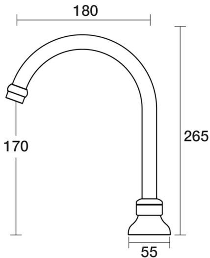
Bell Sink Hob Swivel Outlet D32.032.1.10 - Chrome / Gold
