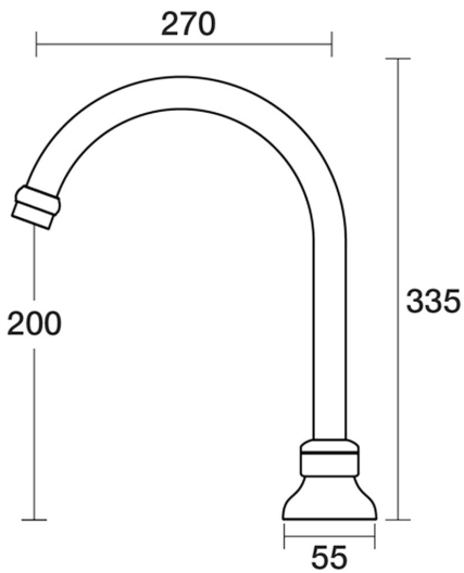
Bell Sink Hob Swivel Outlet X/Large D32.032.2.04 - Chrome / Ivory
