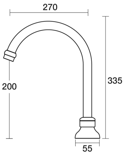
Bell Sink Hob Swivel Outlet X/Large D32.032.2.13 - Gold / White
