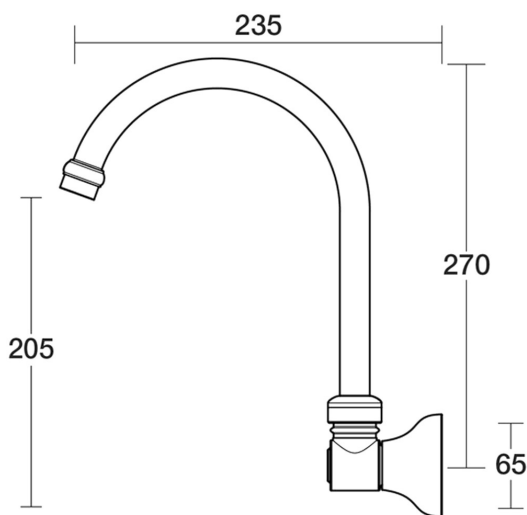
Bell Sink Wall Swivel Outlet D32.034.1.15 - Gold / Apricot
