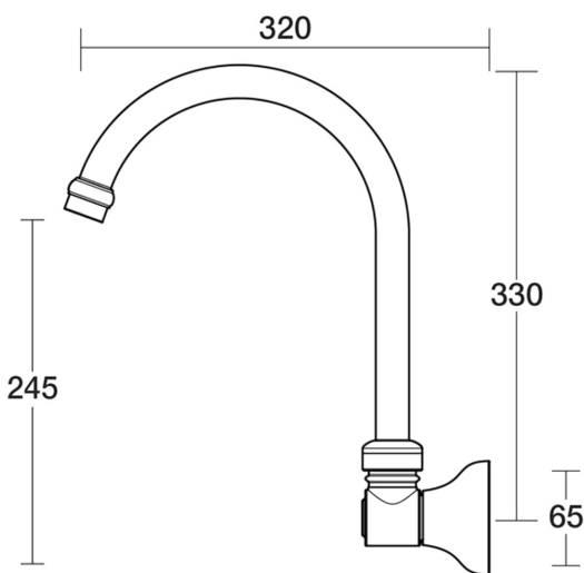
Bell Sink Wall Swivel Outlet X/Large D32.034.2.04 - Chrome / Ivory
