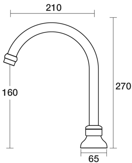
Bell Spa Hob Swivel Outlet D32.042.1.11 - 23k Gold
