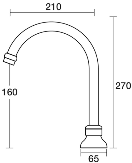
Bell Spa Hob Swivel Outlet D32.042.1.12 - 23k Brushed Gold
