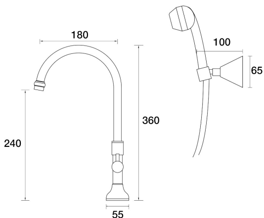
Bell Spa Hob Swivel Outlet Divertor Outlet with Handshower & Bracket Outlet D32.042.2.04 - Chrome / Ivory
