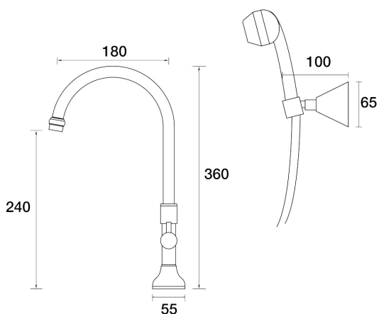
Bell Spa Hob Swivel Outlet Divertor Outlet with Handshower & Bracket Outlet D32.042.2.05 - Chrome / Apricot
