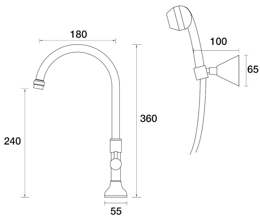
Bell Spa Hob Swivel Outlet Divertor Outlet with Handshower & Bracket Outlet D32.042.2.17 - Gold / Victorian Green
