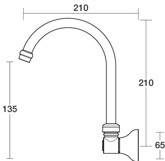
Bell Spa Wall Swivel Outlet D32.044.1.10 - Chrome / Gold
