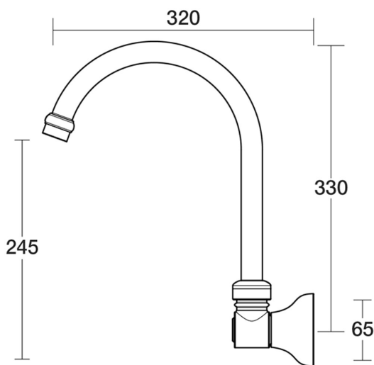
Bell Spa Wall Swivel Outlet X/Large D32.044.2.15 - Gold / Apricot
