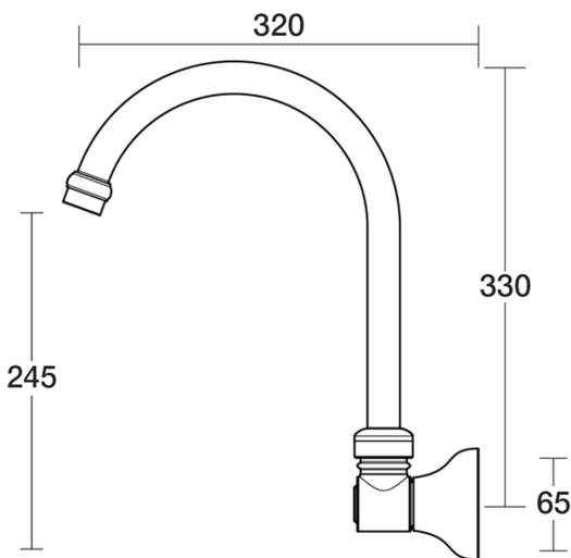
Bell Spa Wall Swivel Outlet X/Large D32.044.2.19 - 23k Brushed Brass Gold
