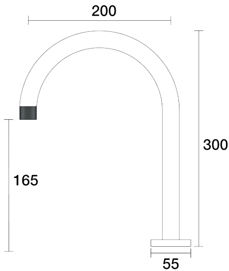
IDK Sink Hob Swivel Outlet D38.032.1.01 - Chrome
