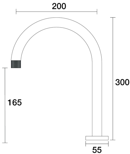
IDK Sink Hob Swivel Outlet D38.032.1.12 - 23k Brushed Gold
