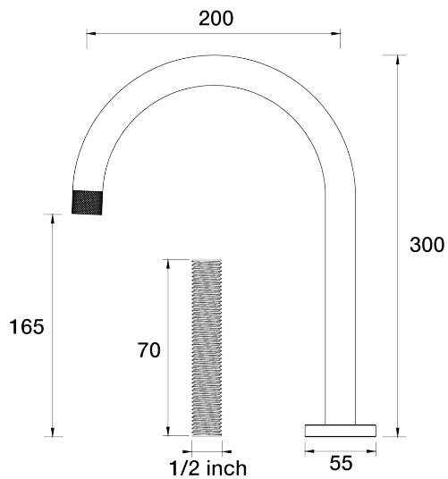
IDK Sink Hob Swivel Outlet For Basin Application ( With Male Thread Nipple) D38.032.2.01 - Chrome
