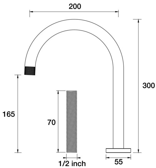
IDK Sink Hob Swivel Outlet For Basin Application ( With Male Thread Nipple) D38.032.2.01 - Chrome
