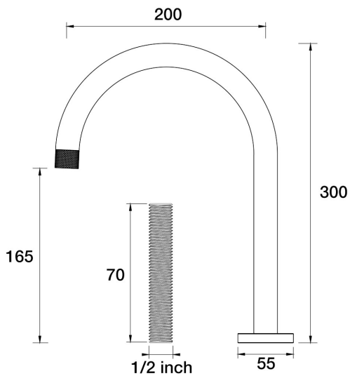
IDK Sink Hob Swivel Outlet For Basin Application ( With Male Thread Nipple) D38.032.2.02 - Brushed Chrome
