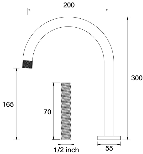
IDK Sink Hob Swivel Outlet For Basin Application ( With Male Thread Nipple) D38.032.2.32 - Midnight Black
