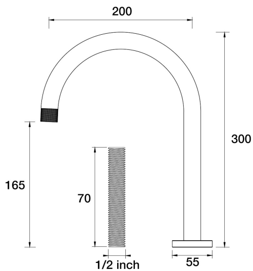
IDK Sink Hob Swivel Outlet For Basin Application ( With Male Thread Nipple) D38.032.2.34 - Matt Black
