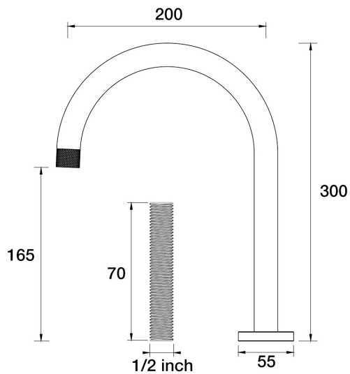
IDK Sink Hob Swivel Outlet For Basin Application ( With Male Thread Nipple) D38.032.2.40 - Rumbled Brass
