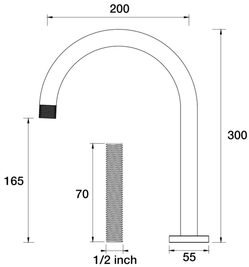
IDK Sink Hob Swivel Outlet For Basin Application ( With Male Thread Nipple) D38.032.2.42 - Brushed Copper
