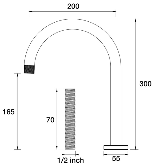
IDK Sink Hob Swivel Outlet For Basin Application ( With Male Thread Nipple) D38.032.2.47 - Luminick
