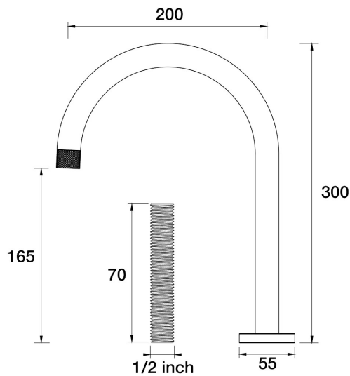
IDK Sink Hob Swivel Outlet For Basin Application ( With Male Thread Nipple) D38.032.2.75 - Forest Mist
