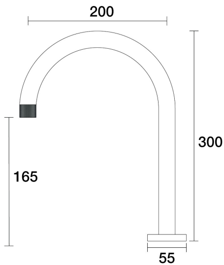
IDK Spa Hob Swivel Outlet D38.042.1.24 - Brushed Gunmetal
