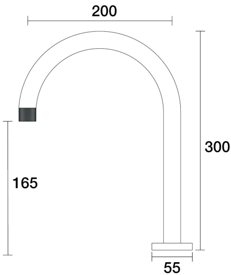
IDK Spa Hob Swivel Outlet D38.042.1.52 - Burnished
