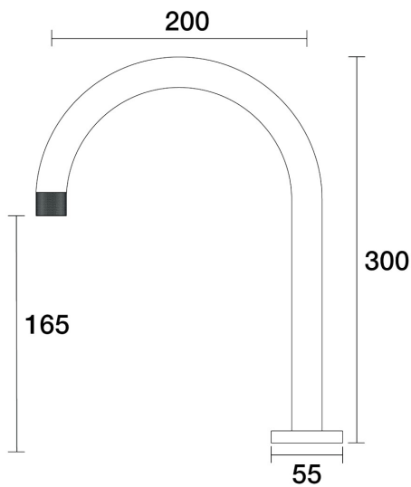
IDK Spa Hob Swivel Outlet D38.042.1.67 - Vintage Brass
