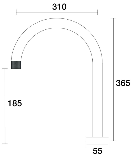
IDK Spa Hob Swivel Outlet X/Large D38.042.2.32 - Midnight Black
