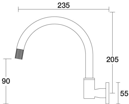
IDK Spa Wall Swivel Outlet D38.044.1.01 - Chrome
