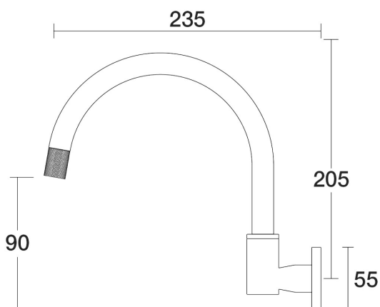
IDK Spa Wall Swivel Outlet D38.044.1.41 - Brushed Brass
